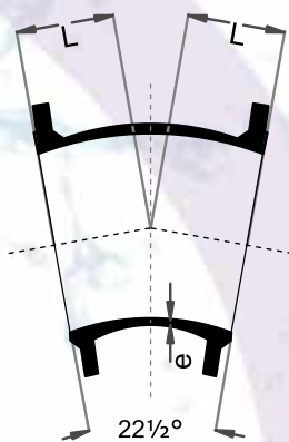
Double Flanged 22 1/2° Bend
